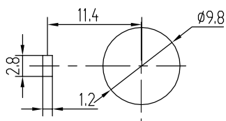
Recommended Panel Cutout Front View Plastic Bushing
