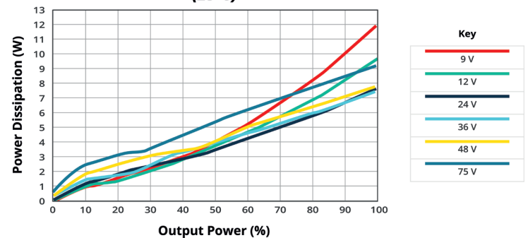
POWER DISSIPATION VS OUTPUT POWER PRQE75W-E12-S12-D (25°C)
