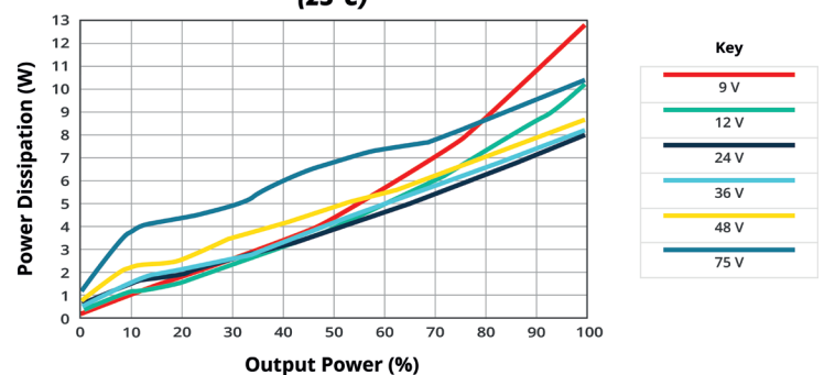
POWER DISSIPATION VS OUTPUT POWER PRQE75W-E12-S15-D (25°C)
