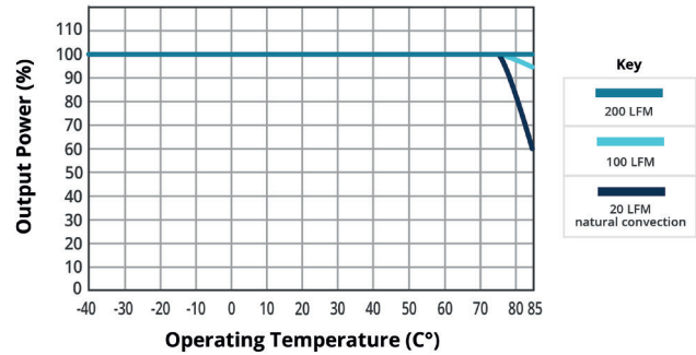
PRQ75W-Q48-S24-B-D (Base plate version) TEMPERATURE DERATING CURVE ( V_{in} = 24\text{ V} )
