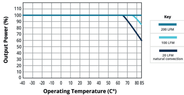
PRQ75W-Q48-S24-D TEMPERATURE DERATING CURVE ( V_{in} = 24\text{ V} )
