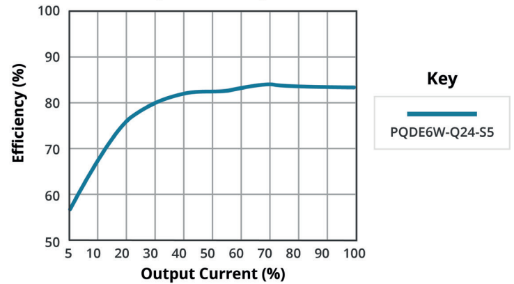
EFFICIENCY VS OUTPUT LOAD ( V_{in} = 24 \text{ Vdc} )
