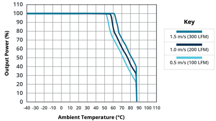
TEMPERATURE DERATING CURVE (with heatsink)
