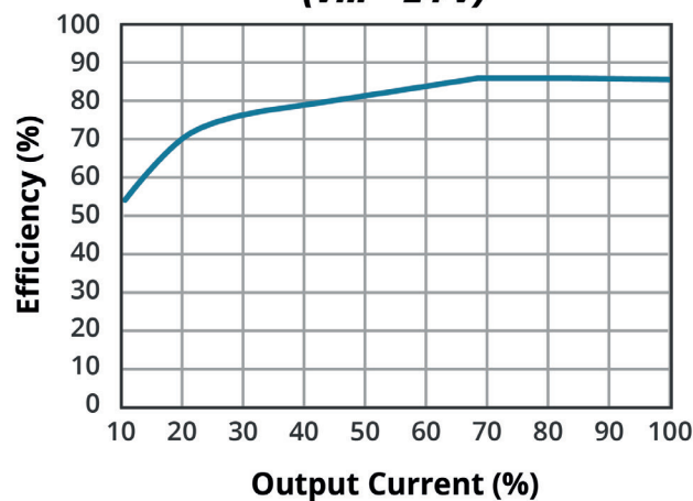
EFFICIENCY VS OUTPUT LOAD PESE2-S24-S5-M (Vin = 24 V)
