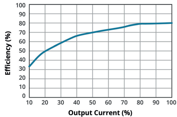
EFFICIENCY VS OUTPUT LOAD ( V_{in} = 24V )
