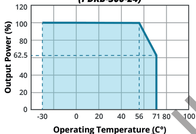
TEMPERATURE DERATING CURVE (PDRB-300-24)
