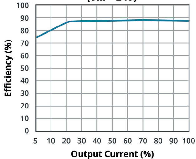
EFFICIENCY VS OUTPUT LOAD PDQE15-Q24-D5-U (Vin = 24V)
