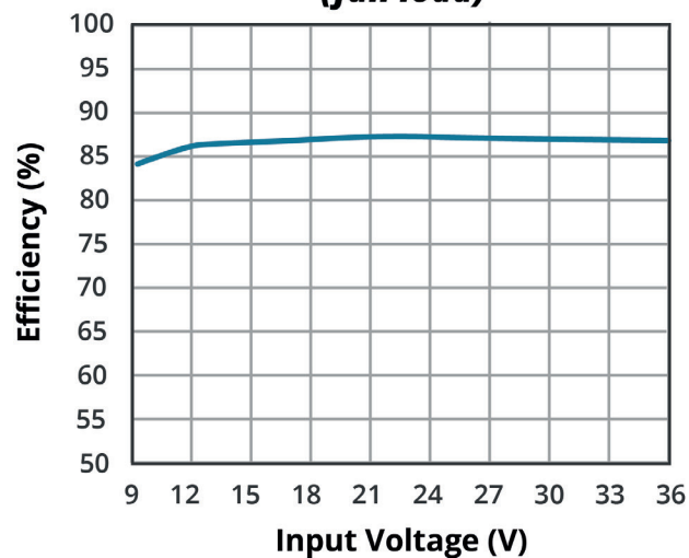
EFFICIENCY VS INPUT VOLTAGE PDQE15-Q24-D5-U (full load)
