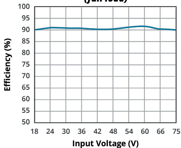
EFFICIENCY VS INPUT VOLTAGE PDQE15-Q48-D24-U (full load)
