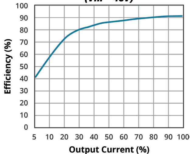
EFFICIENCY VS OUTPUT LOAD PDQE15-Q48-S5-U (Vin = 48V)
