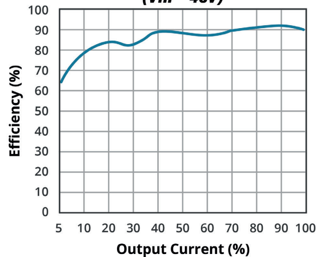
EFFICIENCY VS OUTPUT LOAD PDQE15-Q48-D24-U (Vin = 48V)
