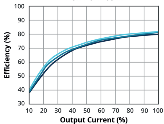
EFFICIENCY VS OUTPUT LOAD PCN1-S12-S5-M
