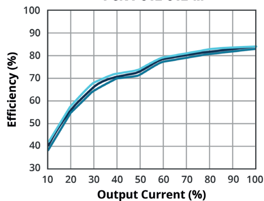
EFFICIENCY VS OUTPUT LOAD PCN1-S12-S12-M
