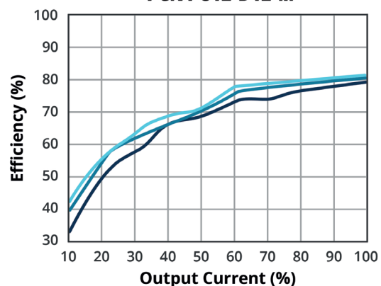
EFFICIENCY VS OUTPUT LOAD PCN1-S12-D12-M
