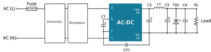
PBO-8 series additional circuits design reference
