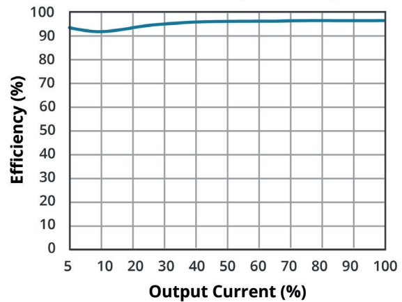
EFFICIENCY VS OUTPUT LOAD P7815-2000-S (Vin = 24 V)
