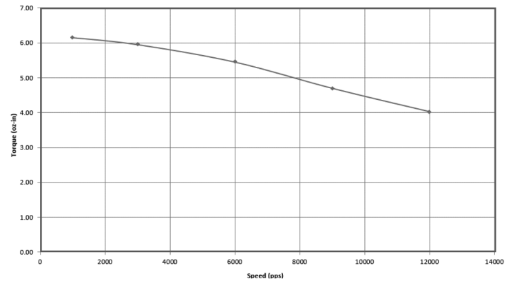
CUI Devices P/N NEMA14-10-080-AMT112S Lin Engineering P/N WD-3518X-08 (1.8 Step Motor) 24 Vdc, 0.35 Amp/Phase, R208, 1/2 Stepping
