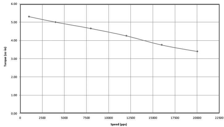
CUI Devices P/N NEMA14-10-040-AMT112S Lin Engineering P/N WD-3518X-04 (1.8 Step Motor) 24 Vdc, 0.45 Amp/Phase, R208, 1/2 Stepping
