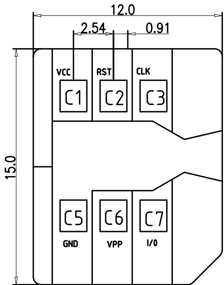
MICRO SIM
