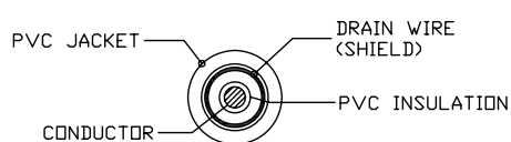
See Table 1 SECTIONAL DRAWING
