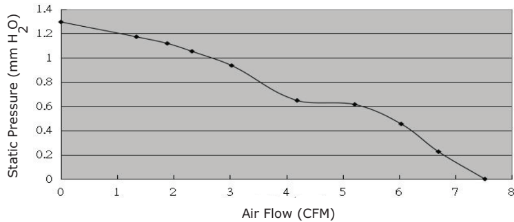
CFM-5010B-135-215
