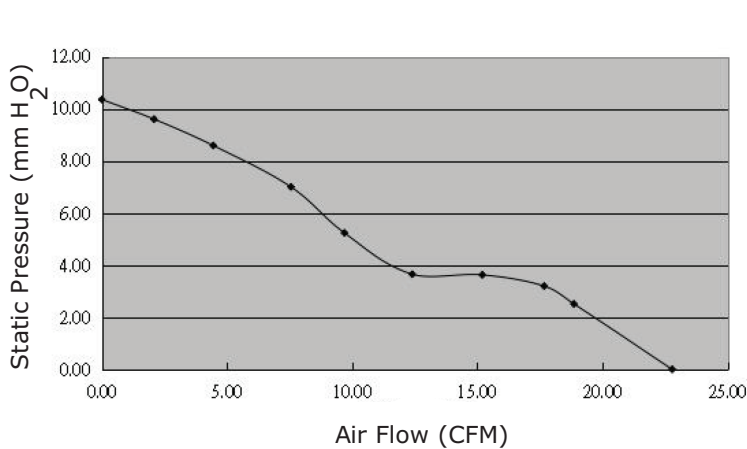
CFM-5020B-275-416
