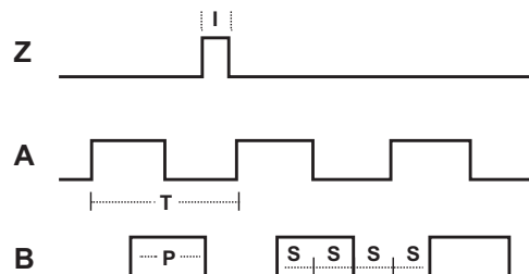
Figure 1 Quadrature signals with index showing counter-clockwise rotation
