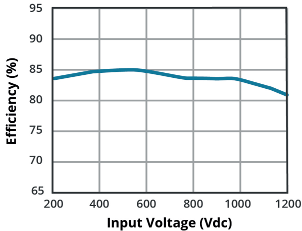
EFFICIENCY VS INPUT VOLTAGE AE40-EW-S12-DIN
