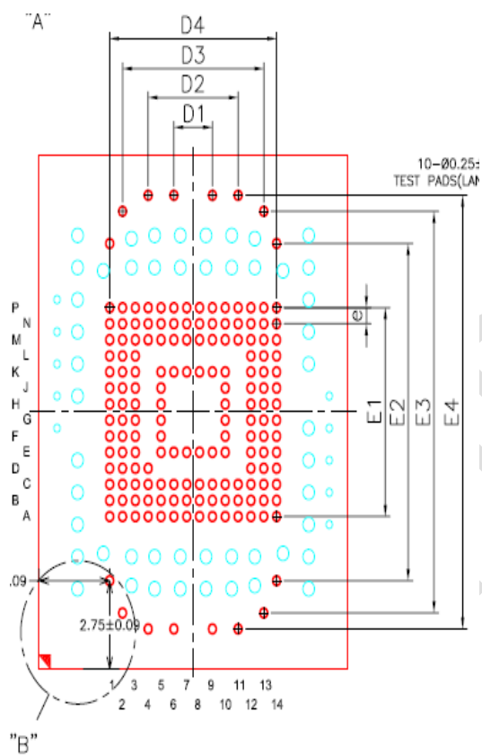
Figure 4b- INAND Specification Top and Side View (Detail A)
