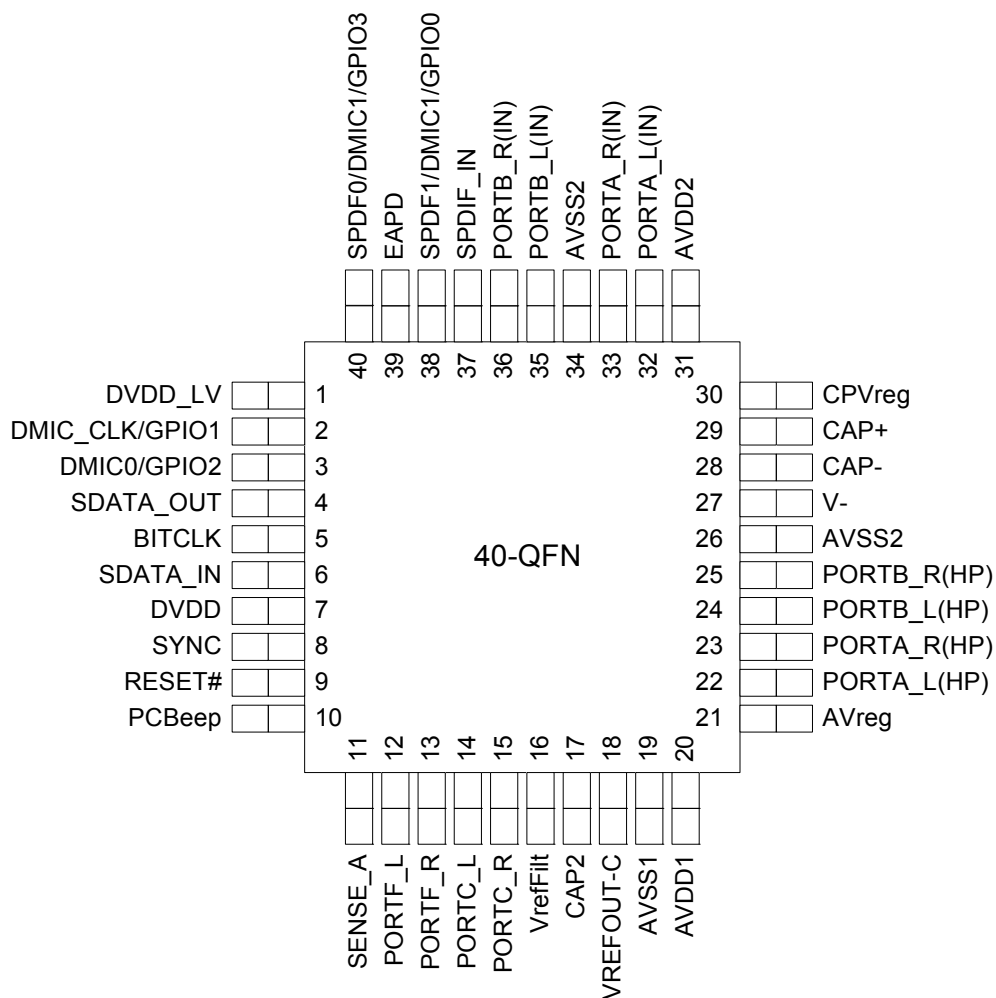
Figure 15. 40-Pin Pinout
