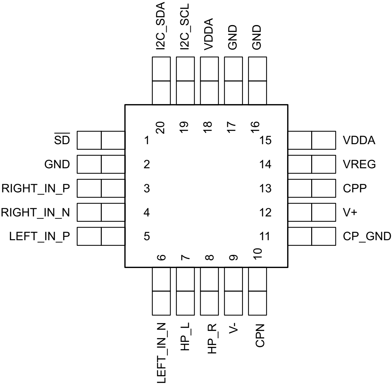
Figure 9. TSDP11xx 20-Pin QFN Pinout
