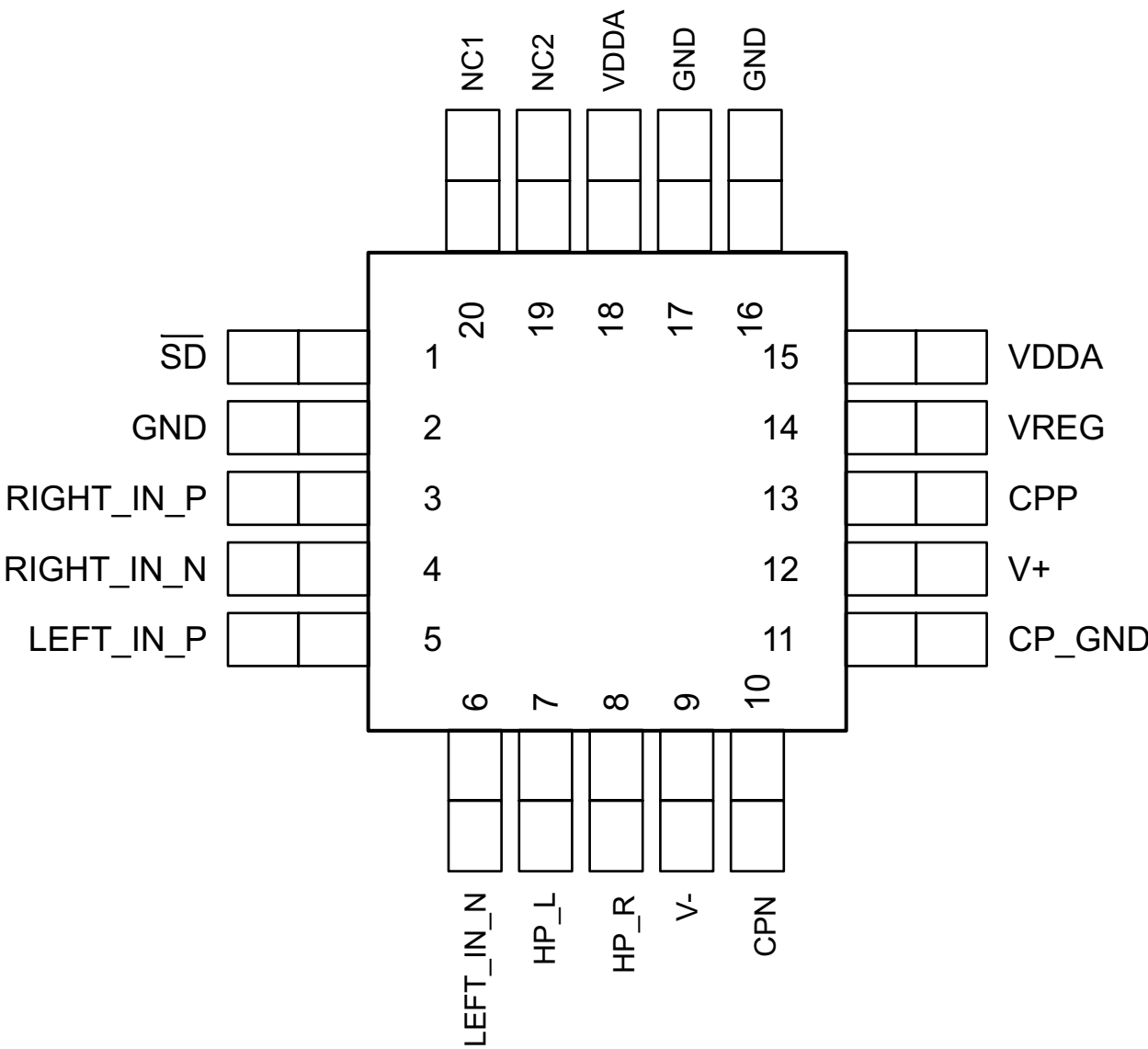
Figure 8. TSDP10xx 20-Pin QFN Pinout
