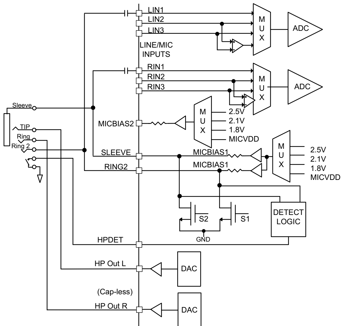
Figure 39. Pin Connection Diagram for 4 Terminal OMTP/CTIA Headset Support with isolated switch
