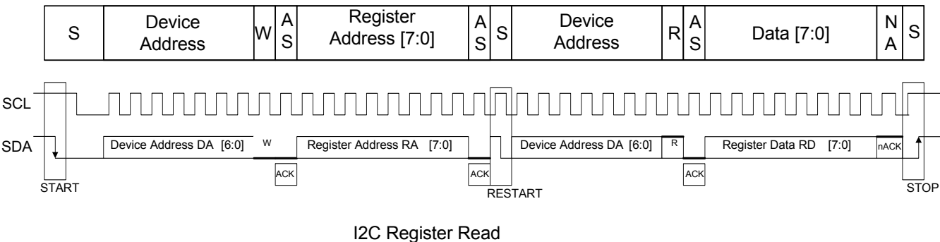
Figure 30. Page Register Single Byte Read Cycle
