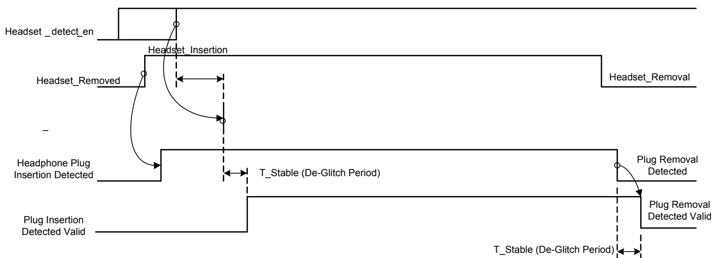
Figure 37. Headset present in jack when Combo-jack detection is enabled
