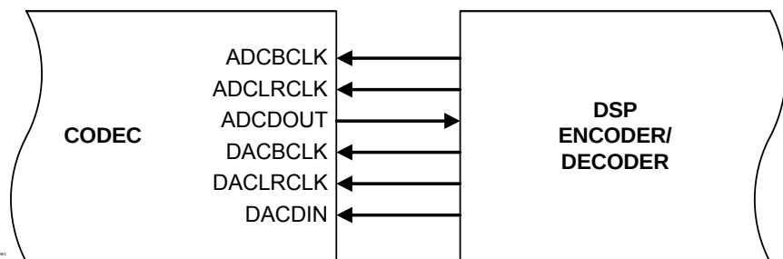
Figure 23. Slave mode
