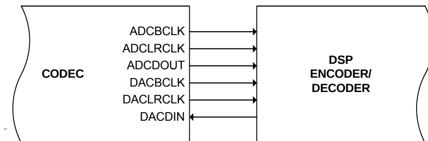
Figure 22. Master mode
