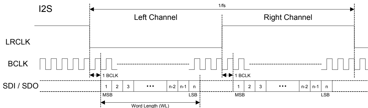
Figure 27. I 2 S Justified Audio Interface (assuming n-bit word length)
