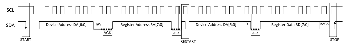
Figure 31. Read Cycle
