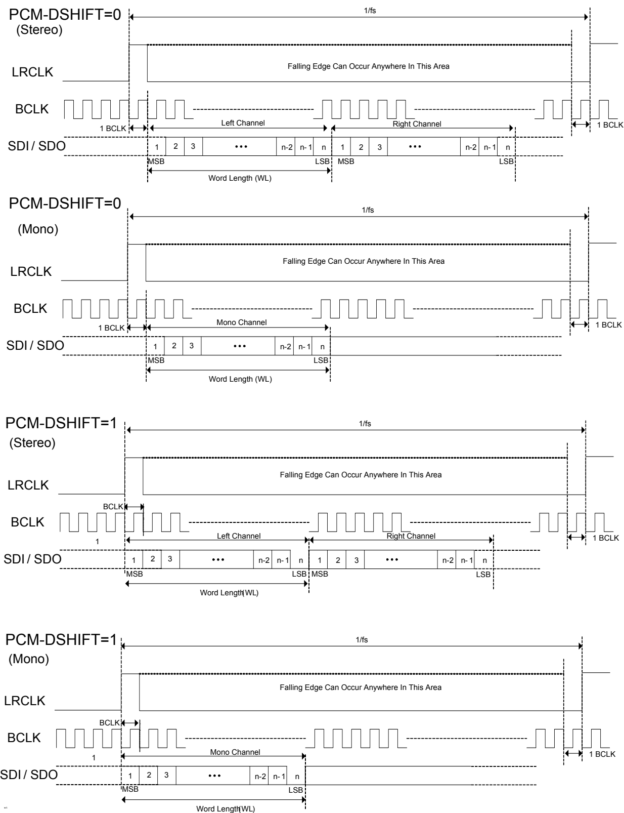
Figure 24. PCM Audio Interface
