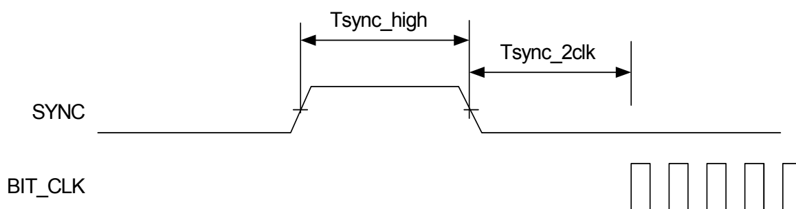
Figure 3. Warm Reset Timing
