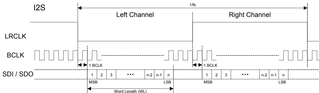
Figure 16. I 2 S Justified Audio Interface (assuming n-bit word length)
