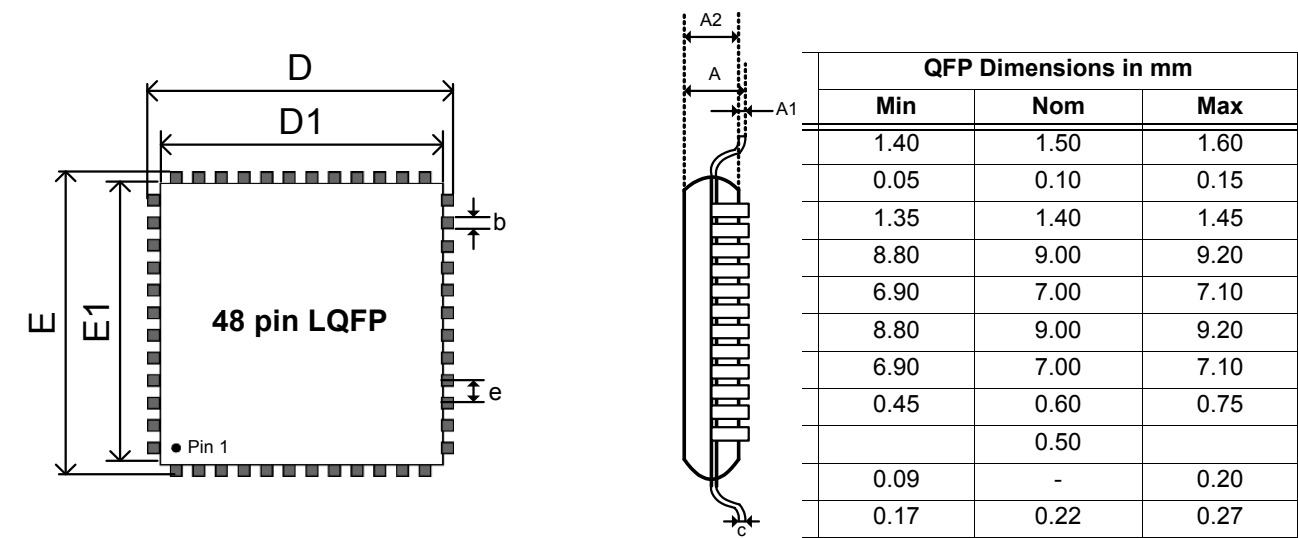
Figure 14. 48-pin QFP Package Drawing
