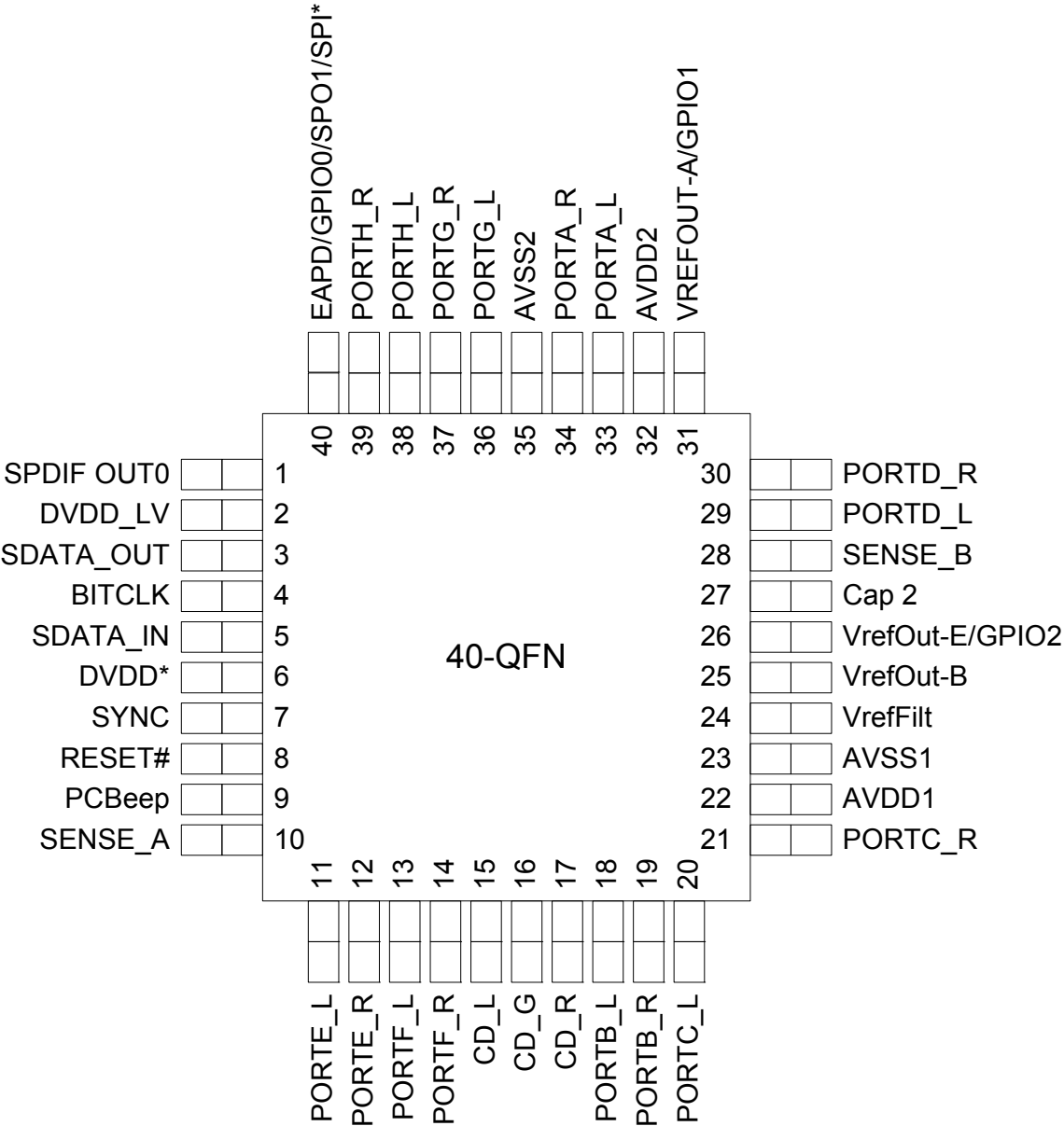
Figure 17. Pin Assignment
