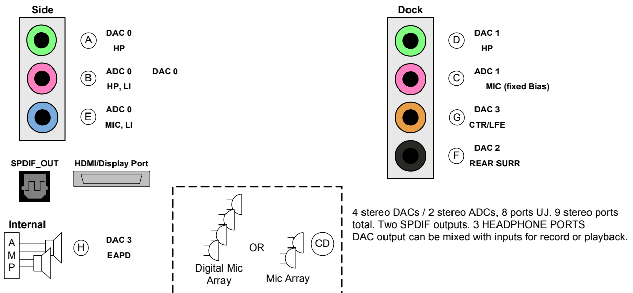
Figure 13. Port Configurations
