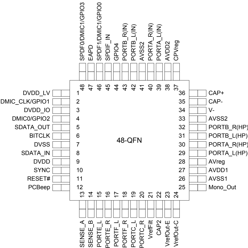
Figure 14. 48-Pin Pinout
