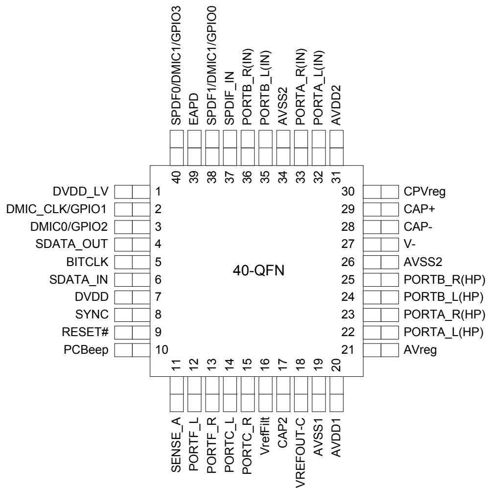
Figure 15. 40-Pin Pinout
