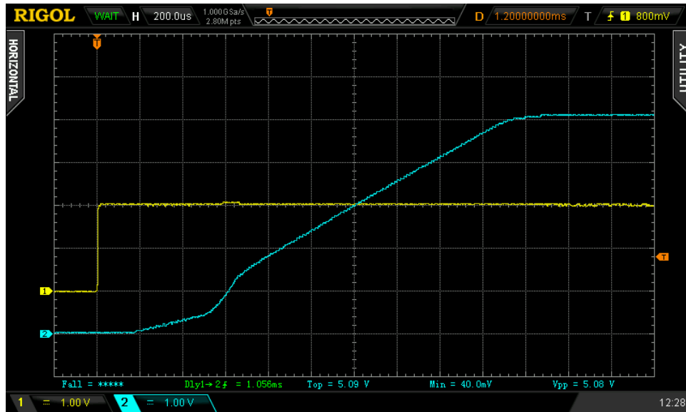
Figure 2. A SLG59M1713V with C_{SLEW} set to 4nF and 470μF for C_{LOAD} . C_{LOAD} -to- C_{SLEW} ratio is greater than 33,600. Note that the internal SCL monitor's been triggered and V_{OUT(SR)} is reduced until V_{OUT} reaches ~0.3V.
