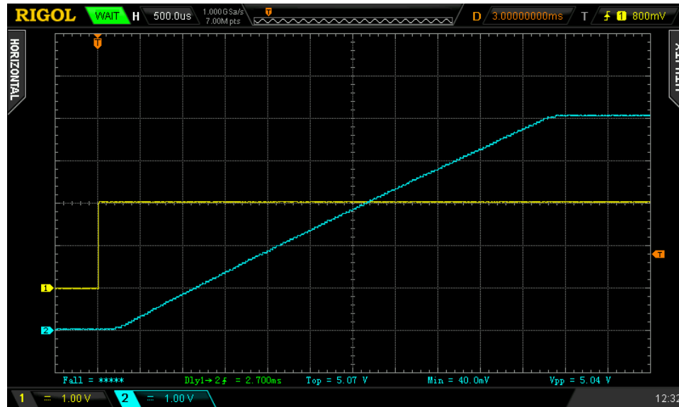
Figure 3. A SLG59M1713V with C_{SLEW} set to 15nF and 470μF retained for C_{LOAD} . C_{LOAD} -to- C_{SLEW} ratio is smaller than 33,600. Note smooth V_{OUT} transition.
