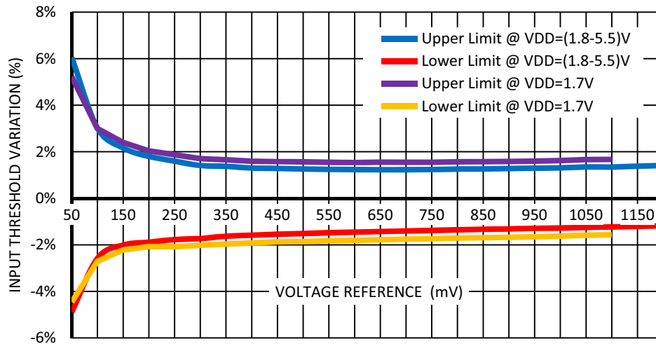
Figure 30. Typical Input Threshold Variation (including Vref variation, ACOMP offset) vs. Voltage reference at room temperature, LBW Mode – Disable, Vhys=0 mV.
