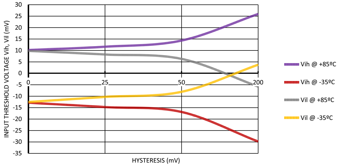
Figure 33. Input Threshold Voltage V_{ih} , V_{il} vs. Hysteresis at V_{DD} = 5.5 V, V_{ref} = 1000 mV. Gain = 1
