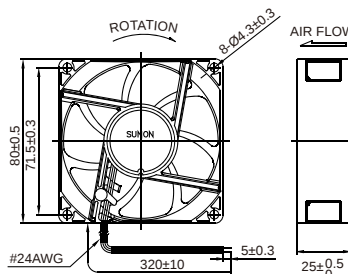
■ External dimensions(mm)
