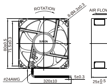
■ External dimensions(mm)
