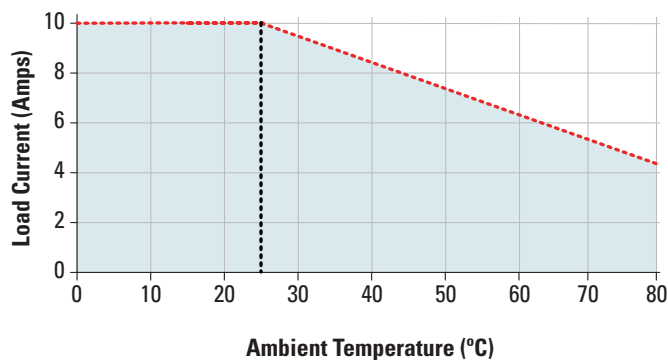
Figure 1 Convection Cooling
