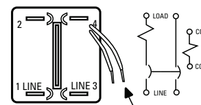
Two Pole (1 pole relay)
