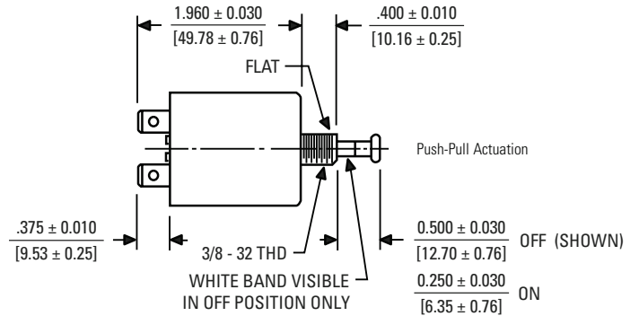
Push-Pull, Two Pole
