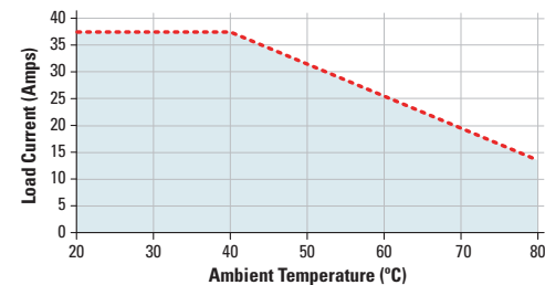
HS172 w/50 Amps single channel SSR
