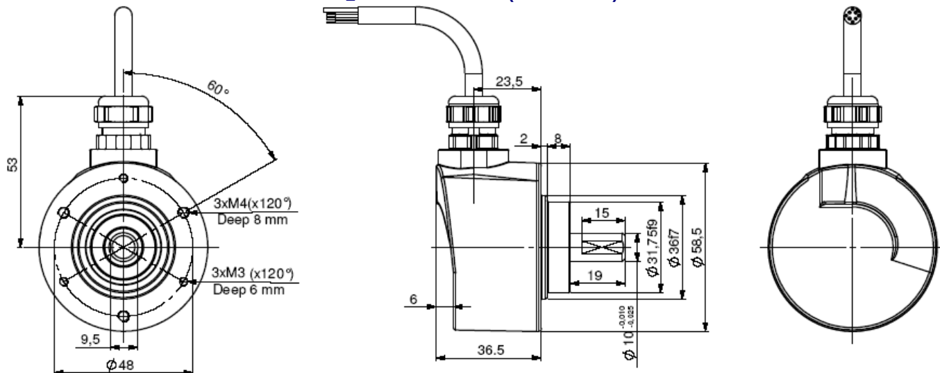
CHM5_06 connection S6R (radial M23), flange 9500/003* mounted on the body
