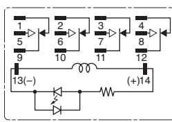
4PDT
