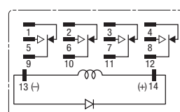
4PDT
