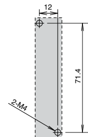
Mounting Hole Layout (M4 Mounting Screws)
