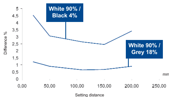
Laser background suppression
