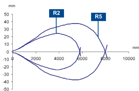
Polarized retroreflex
