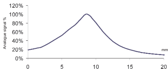
Contrast sensor
