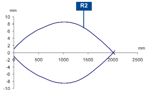
Polarized retroreflex for transparents - T53
