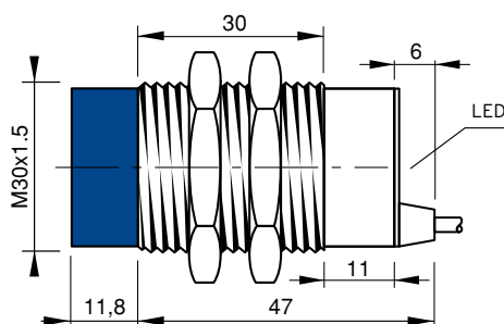
CABLE VERSION
