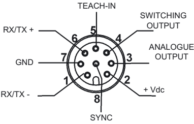
RECEIVER (RX)
