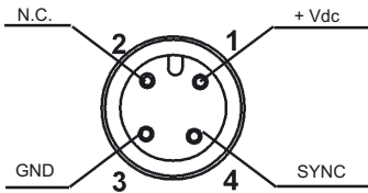
EMITTER (TX)
