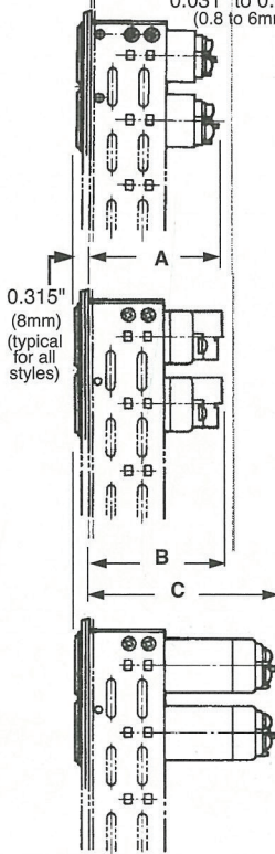
Panel Thickness using mounting clips 0.031" to 0.236" (0.8 to 6mm)
