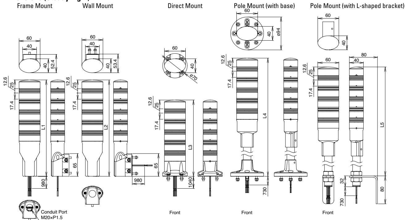
Dimension Table
