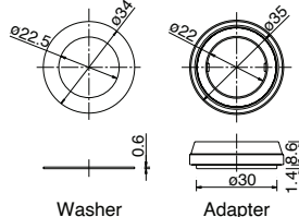
Washer
