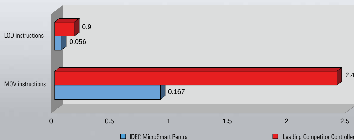
MicroSmart Pentra Slim CPU Speed Comparison (μsecs)
