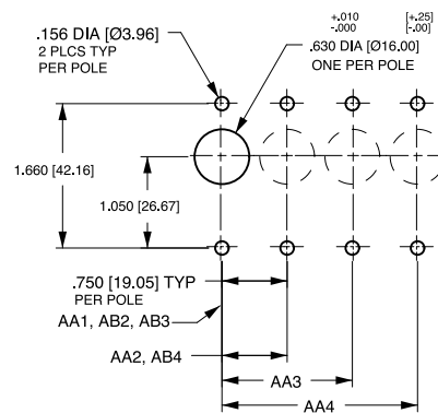
PANEL CUTOUT DETAIL
