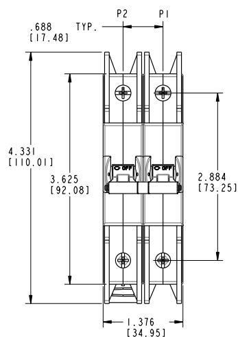
MULTIPLE POLES WITH AUXILIARY SWITCH ( PENDING ) (PLUG-IN TERMINAL BLOCK)
