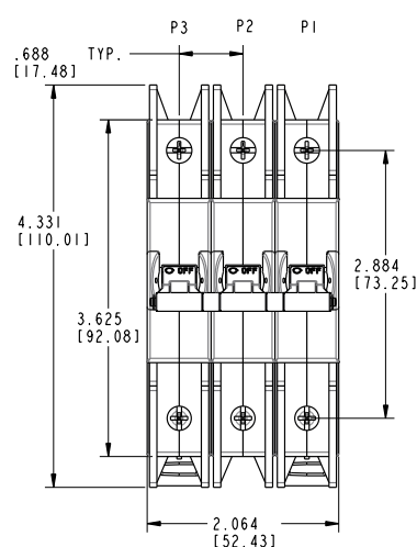
MULTIPLE POLES WITH AUXILIARY SWITCH ( PENDING ) (PLUG-IN TERMINAL BLOCK)
