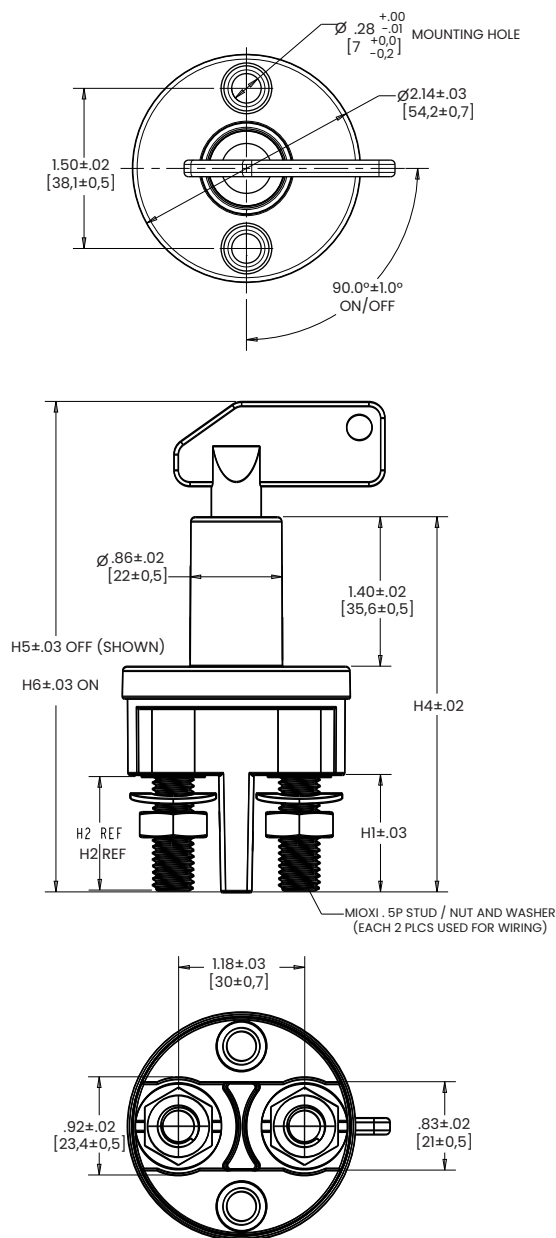
BDI SWITCH WITH KEY
