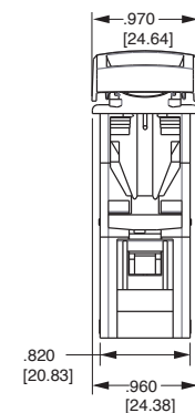
10 TERMINAL BASE W/O BARRIERS
